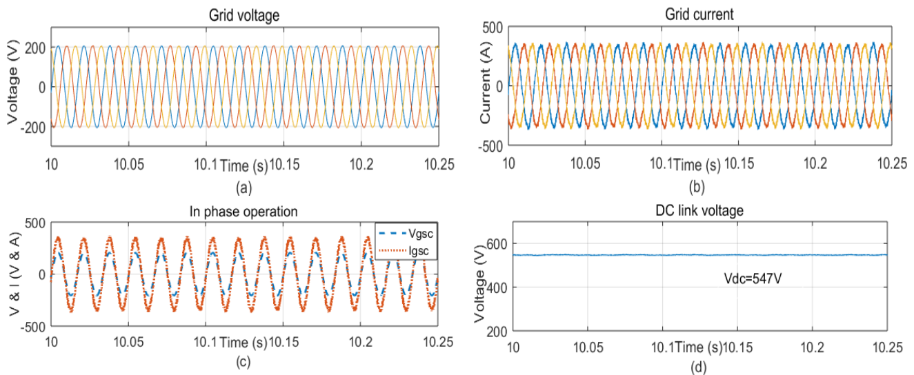
Fig.6. Simulation result for both wind and PV are absent
