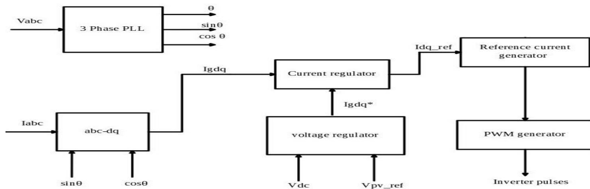
Fig.2 field oriented control algorithm for GSC
