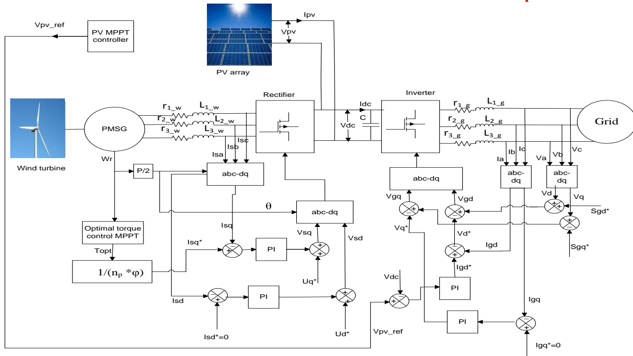
Fig.1Block diagram of proposed PV-wind grid connected system
