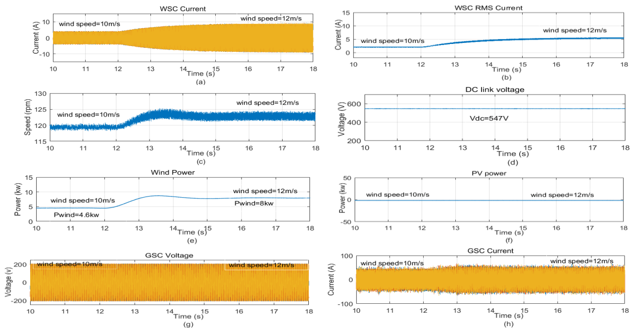
Fig.4. Simulation results for PV delivers power to grid
