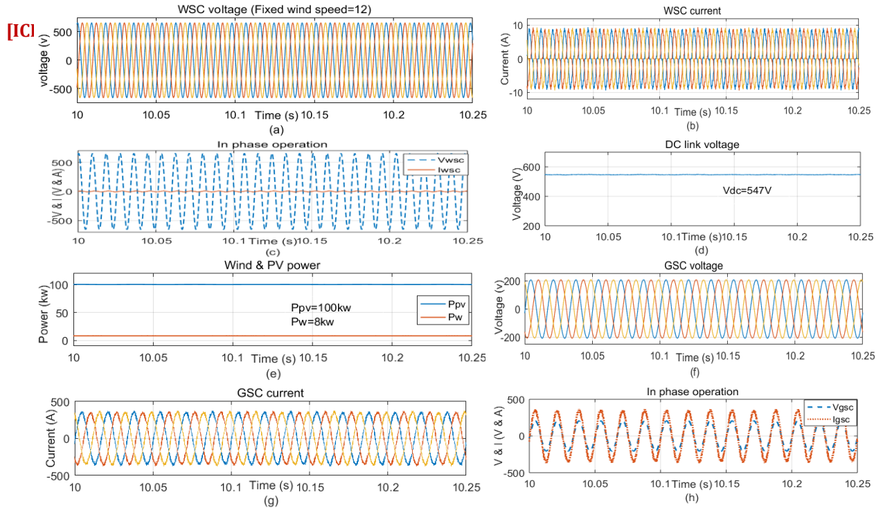
Fig.3. Simulation result for PV and wind delivers power to grid
