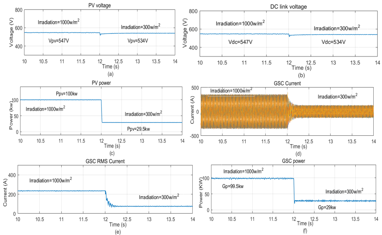
Fig.5. Simulation result for wind delivers power to grid.
